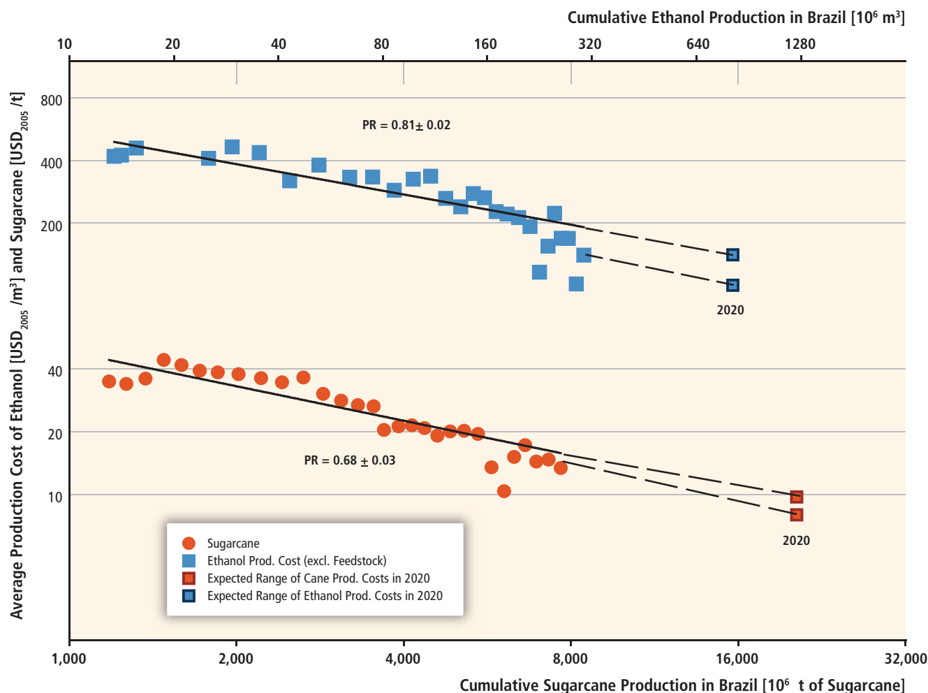
Figure 2.21 | Brazilian sugarcane and ethanol production cost learning curves for between 1975 and 2005 and extrapolated to 2020 (in \text{USD}_{2005} ). Progress ratio ( \text{PR}=1-\text{LR} ) is obtained by best fit to data (van den Wall Bake et al., 2009; reproduced with permission from Elsevier B.V.).
